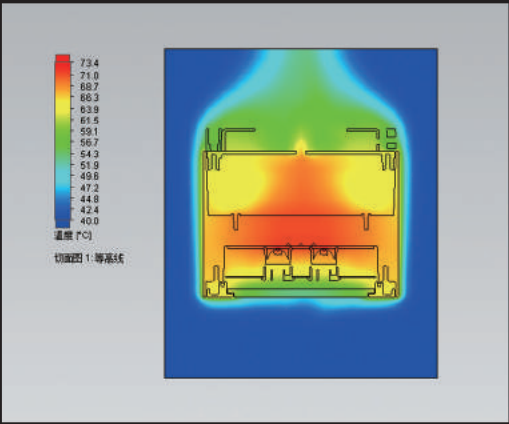
优异的散热性能 Excellent heat dissipation
